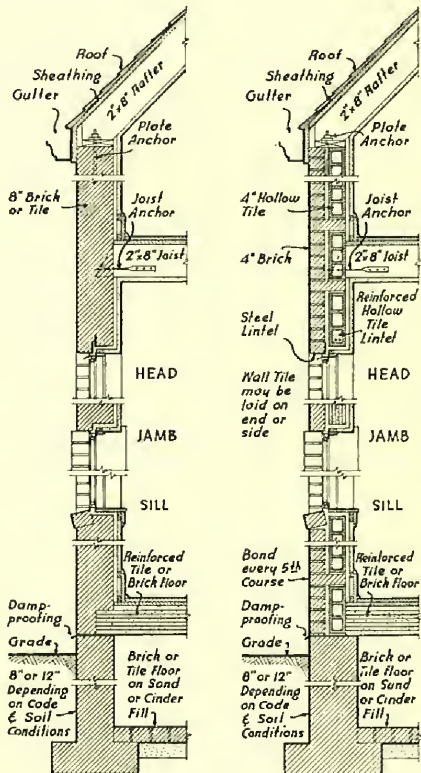
Wall Sections
